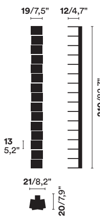
PT WALL 210
