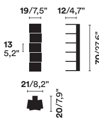
PT WALL 70
