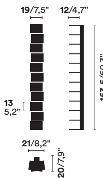
PT WALL 155
